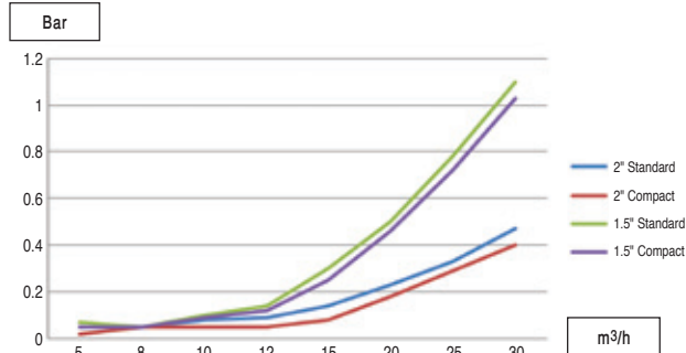
1.5-2" EITAN SCREEN FILTERS HEAD LOSS
